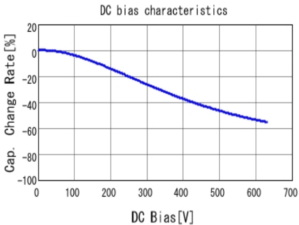
■ GRM31AR72J102KW01 C-DC bias capchange, 25.0degC, AC1V
