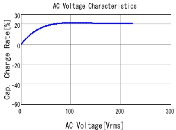
■ GRM31AR72J102KW01 C-AC Voltage capchange, DCOV, 25.0d
