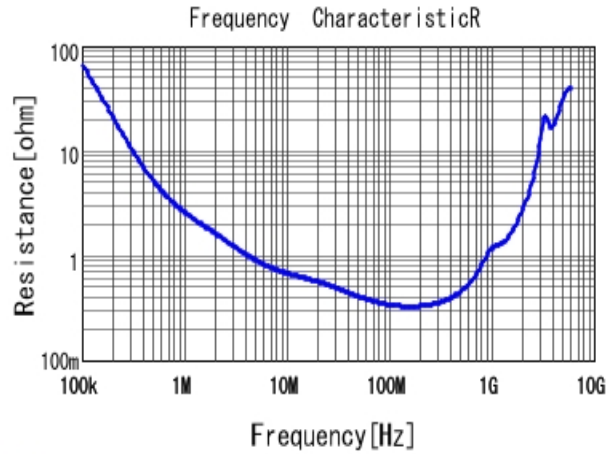
■ GRM31AR72J102KW01 R DCOV, 25degC
