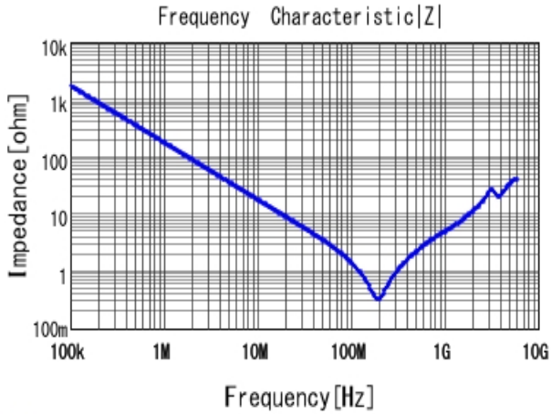
■ GRM31AR72J102KW01 |Z| DCOV, 25degC
