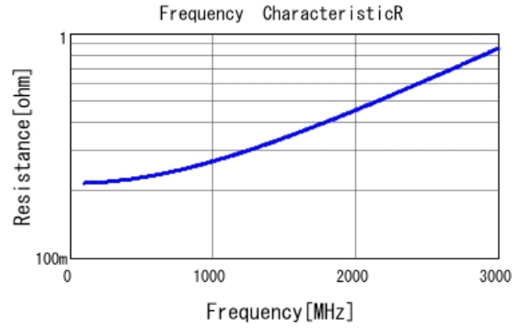
■ GRM31A7U3D100JW31 R DCOV, 25degC
