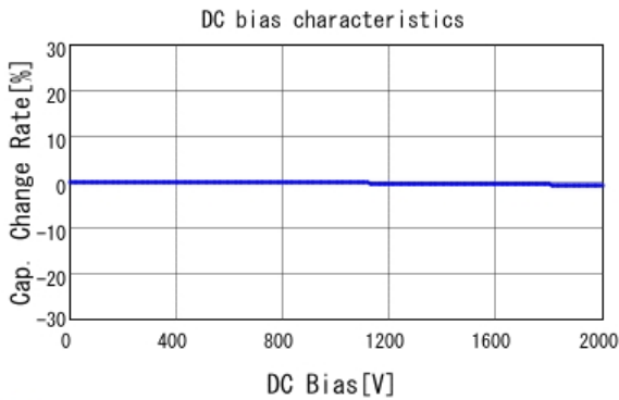
■ GRM31A7U3D100JW31 C-DC bias capchange, 25.0degC, AC1V
