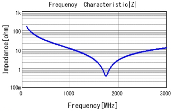
■ GRM31A7U3D100JW31 |Z| DCOV, 25degC
