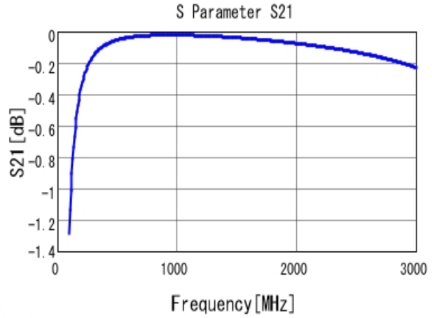
■ GRM31A7U3A270JW31 S21 DCOV, 25degC
