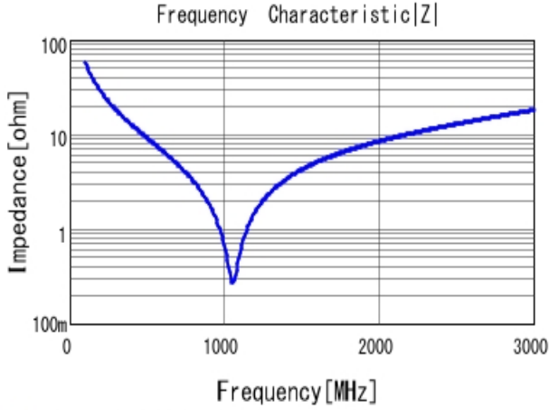
■ GRM31A7U3A270JW31 |Z| DC0V, 25degC
