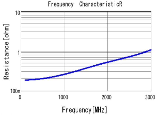
■ GRM31A7U3A270JW31 R DC0V, 25degC
