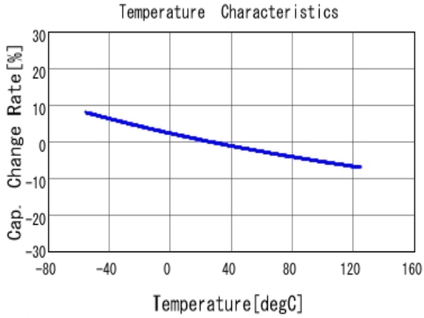
■ GRM31A7U3A270JW31 C-Temp. capchange, DCOV, AC1Vrms
