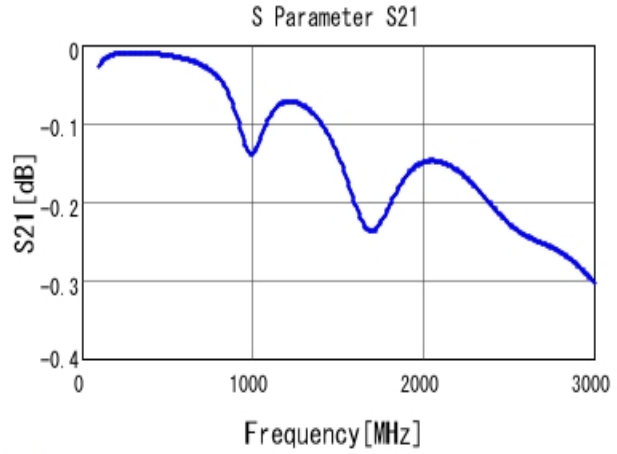
■ GRM31A7U3A221JW31 S21 DCOV, 25degC
