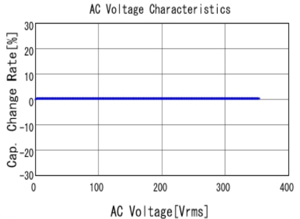
■ GRM31A7U3A221JW31 C-AC Voltage capchange, DCOV, 25.0d
