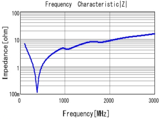
■ GRM31A7U3A221JW31 |Z| DCOV, 25degC
