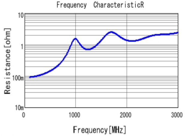
■ GRM31A7U3A221JW31 R DCOV, 25degC
