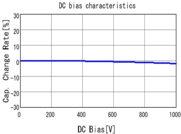
■ GRM31A7U3A221JW31 C-DC bias capchange, 25.0degC, AC1V
