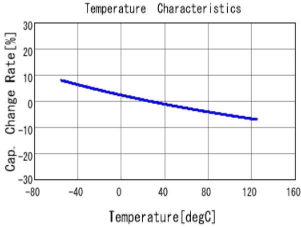
■ GRM31A7U3A221JW31 C-Temp. capchange, DCOV, AC1Vrms
