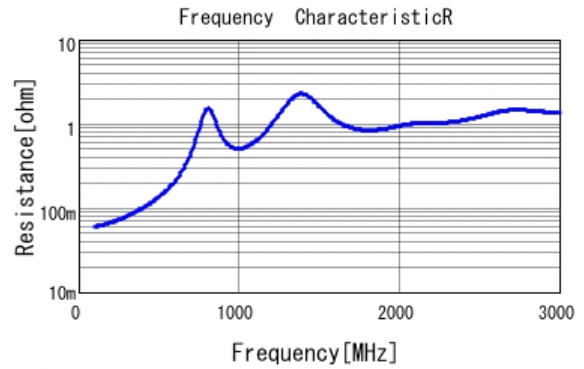
■ GRM31A7U2J331JW31 R DCOV, 25degC
