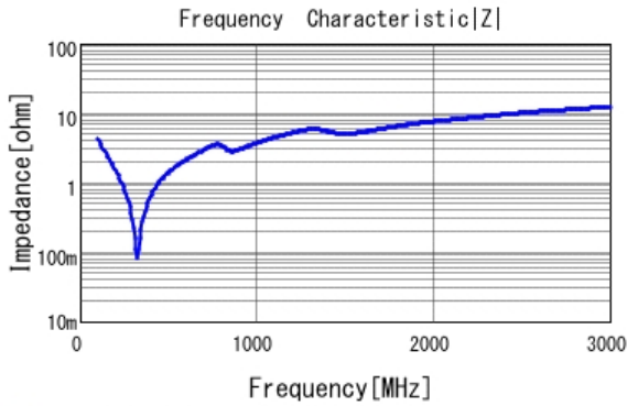
■ GRM31A7U2J331JW31 |Z| DCOV, 25degC
