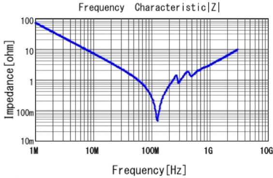
■ GRM31A7U2J222JW31 |Z| DCOV, 25degC
