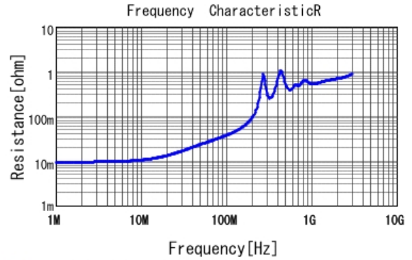
■ GRM31A7U2J222JW31 R DCOV, 25degC
