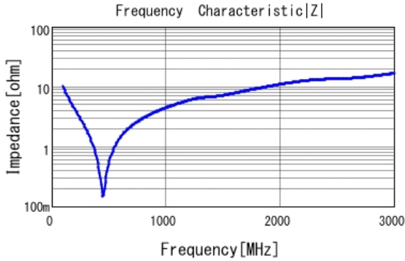
■ GRM31A7U2J151JW31 |Z| DCOV, 25degC
