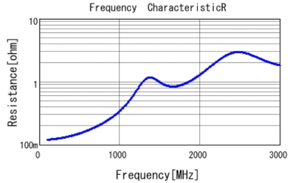
■ GRM31A7U2J151JW31 R DCOV, 25degC
