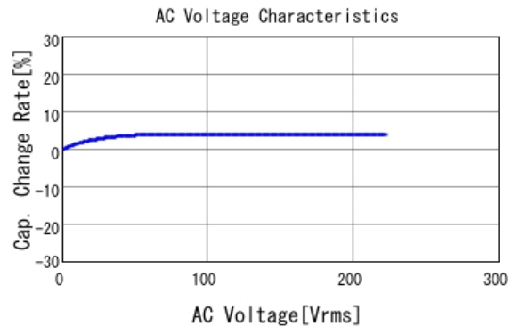
■ GRM31A7U2J151JW31 C-AC Voltage capchange, DCOV, 25.0d
