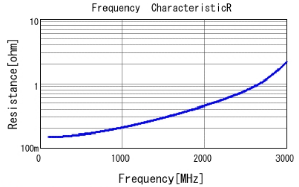
■ GRM31A5C3A470JW01 R DCOV, 25degC
