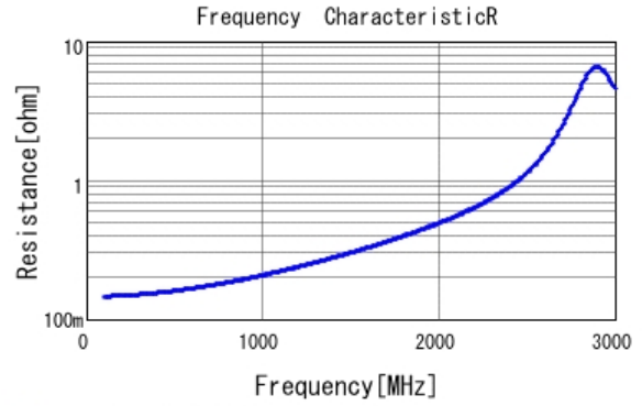
■ GRM31A5C3A390JW01 R DCOV, 25degC
