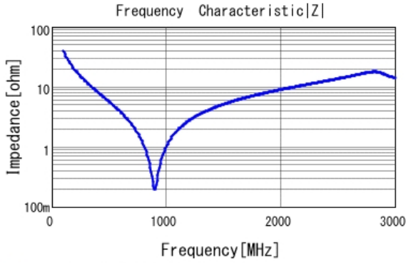
■ GRM31A5C3A390JW01 |Z| DCOV, 25degC
