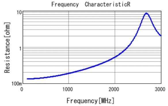
■ GRM31A5C3A330JW01 R DCOV, 25degC
