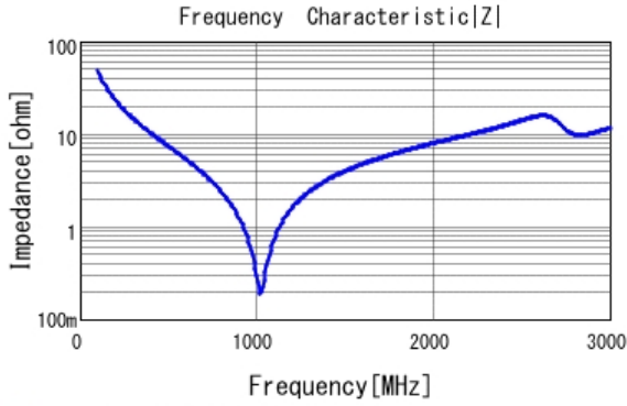
■ GRM31A5C3A330JW01 |Z| DCOV, 25degC
