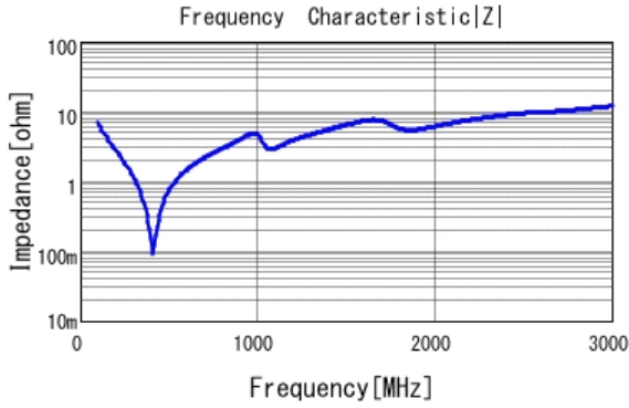
■ GRM31A5C3A221JW01 |Z| DCOV, 25degC
