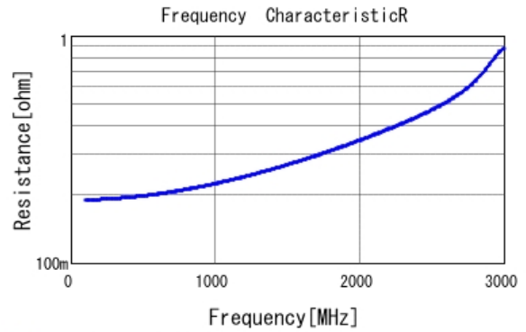
■ GRM31A5C3A100JW01 R DC0V, 25degC
