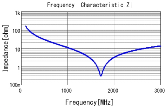
■ GRM31A5C3A100JW01 |Z| DC0V, 25degC
