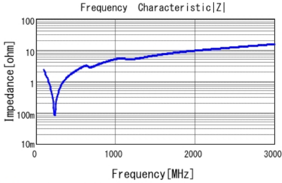
■ GRM31A5C2J561JW01 |Z| DC0V, 25degC
