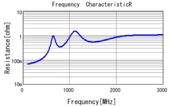
■ GRM31A5C2J561JW01 R DC0V, 25degC
