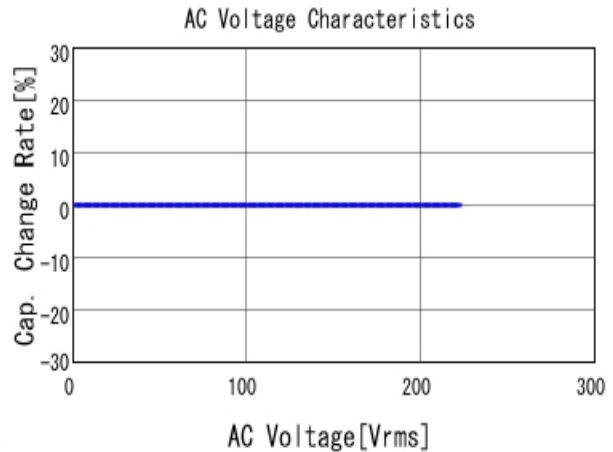
■ GRM31A5C2J471JW01 C-AC Voltage capchange, DCOV, 25.0d
