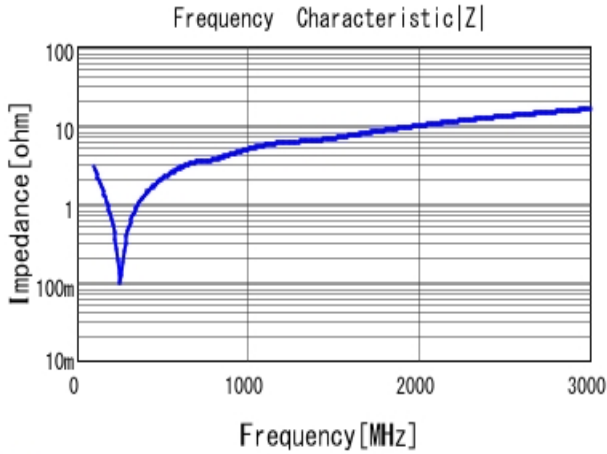
■ GRM31A5C2J471JW01 |Z| DCOV, 25degC
