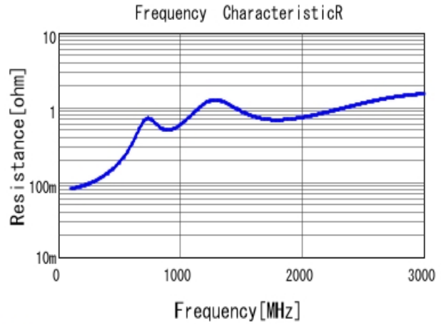
■ GRM31A5C2J471JW01 R DCOV, 25degC
