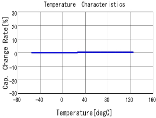
■ GRM31A5C2J471JW01 C-Temp. capchange, DCOV, AC1Vrms
