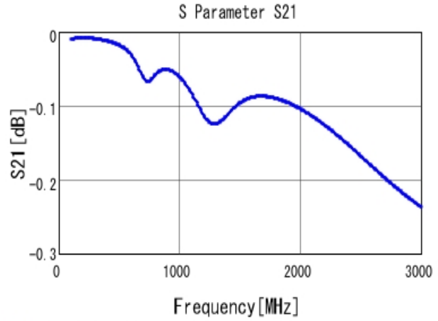
■ GRM31A5C2J471JW01 S21 DCOV, 25degC
