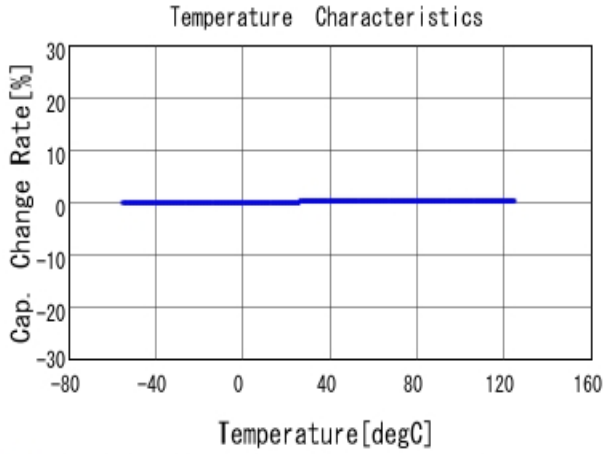
■ GRM31A5C2J470JW01 C-Temp. capchange, DCOV, AC1Vrms
