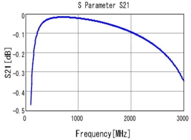
■ GRM31A5C2J470JW01 S21 DCOV, 25degC
