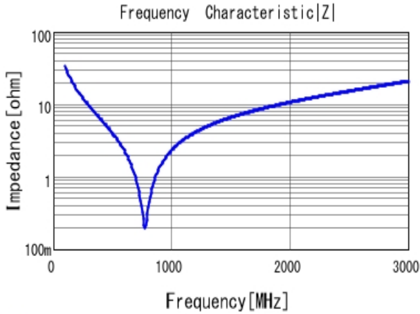
■ GRM31A5C2J470JW01 |Z| DC0V, 25degC
