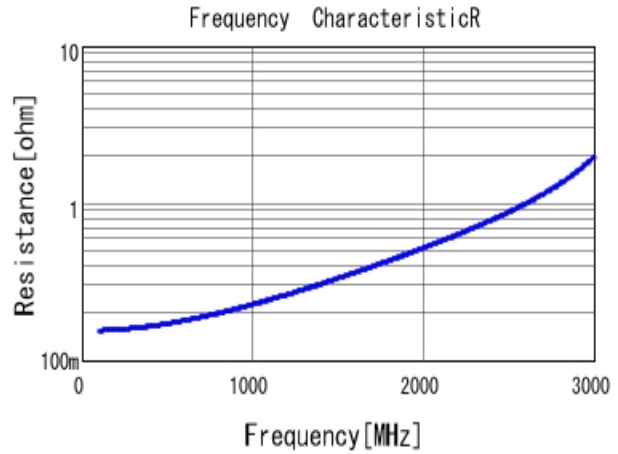
■ GRM31A5C2J470JW01 R DC0V, 25degC
