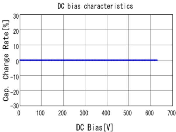
■ GRM31A5C2J470JW01 C-DC bias capchange, 25.0degC, AC1V
