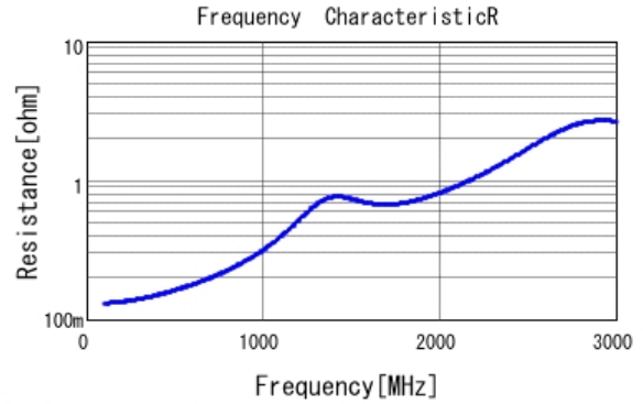
■ GRM31A5C2J221JW01 R DC0V, 25degC
