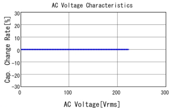
■ GRM31A5C2J221JW01 C-AC Voltage capchange, DC0V, 25.0d
