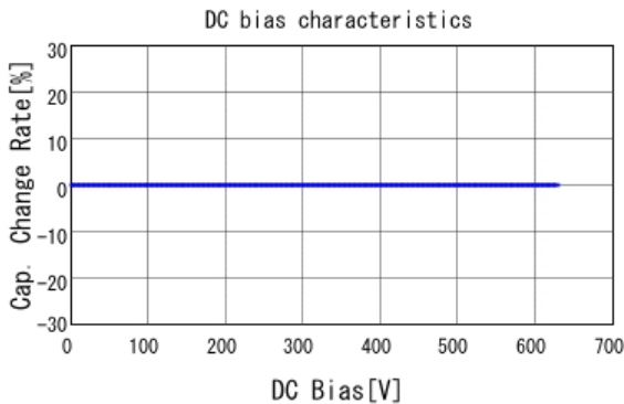
■ GRM31A5C2J221JW01 C-DC bias capchange, 25.0degC, AC1V
