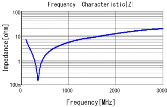
■ GRM31A5C2J221JW01 |Z| DC0V, 25degC
