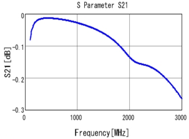
■ GRM31A5C2J121JW01 S21 DCOV, 25degC
