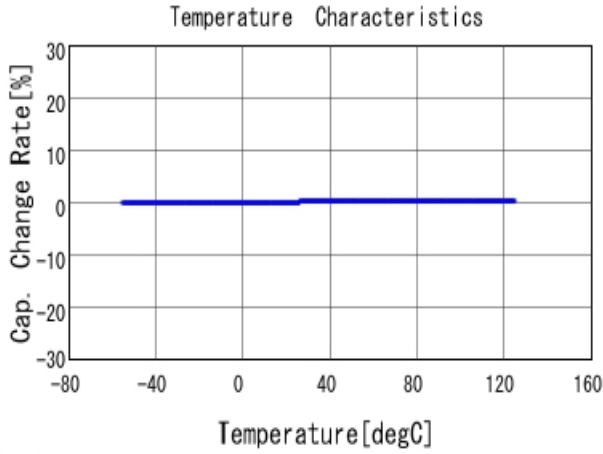
■ GRM31A5C2J121JW01 C-Temp. capchange, DCOV, AC1Vrms
