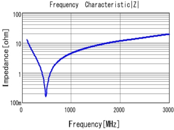
■ GRM31A5C2J121JW01 |Z| DC0V, 25degC
