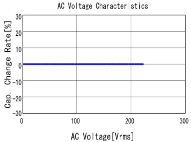
■ GRM31A5C2J121JW01 C-AC Voltage capchange, DC0V, 25.0d
