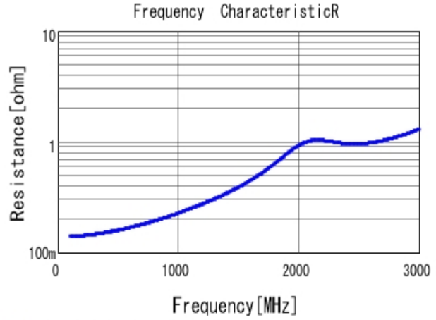
■ GRM31A5C2J121JW01 R DC0V, 25degC
