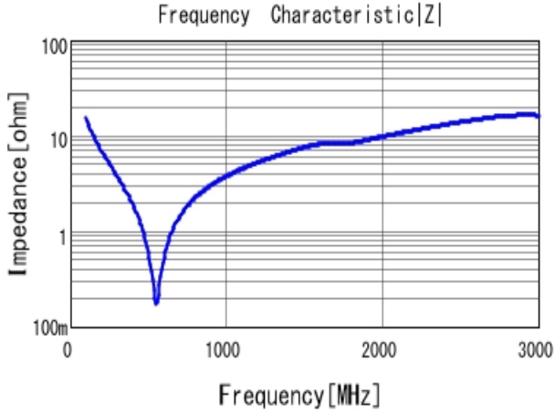
■ GRM31A5C2J101JW01 |Z| DCOV, 25degC
