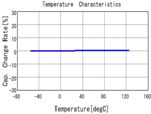
■ GRM31A5C2J101JW01 C-Temp. capchange, DCOV, AC1Vrms
