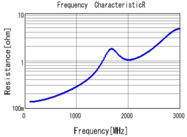
■ GRM31A5C2J101JW01 R DCOV, 25degC
