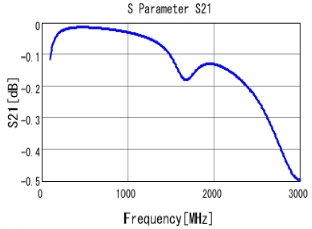
■ GRM31A5C2J101JW01 S21 DCOV, 25degC
