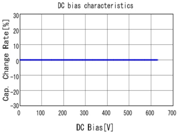
■ GRM31A5C2J101JW01 C-DC bias capchange, 25.0degC, AC1V
