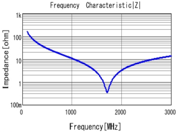
■ GRM31A5C2J100JW01 |Z| DC0V, 25degC
