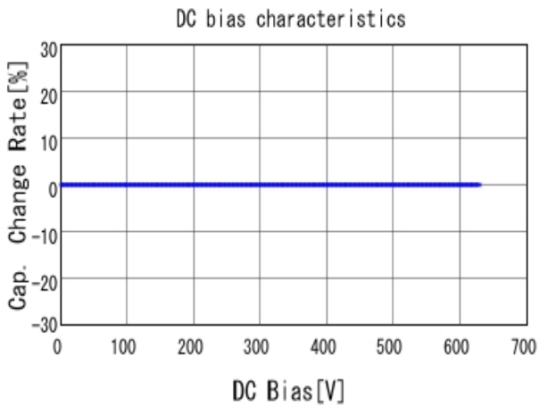
■ GRM31A5C2J100JW01 C-DC bias capchange, 25.0degC, AC1V
