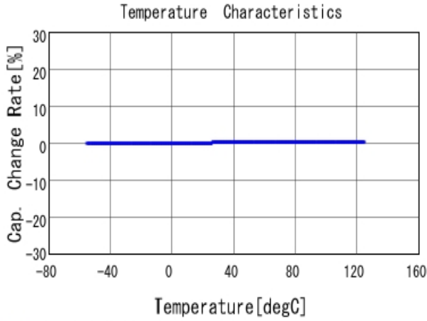
■ GRM31A5C2J100JW01 C-Temp. capchange, DCOV, AC1Vrms
