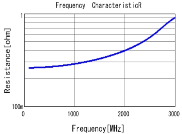
■ GRM31A5C2J100JW01 R DC0V, 25degC
