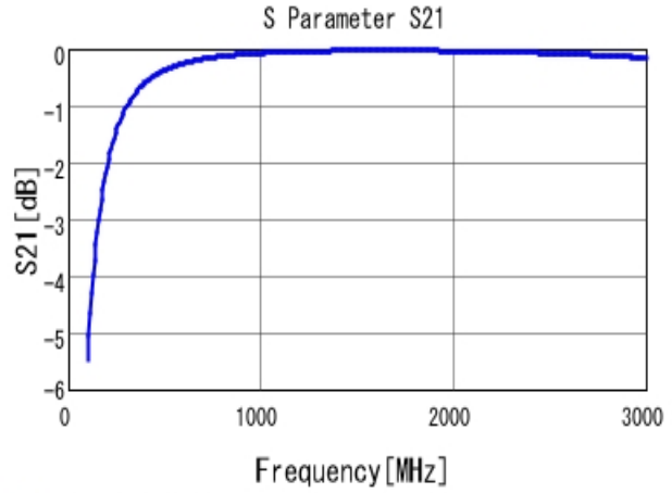
■ GRM31A5C2J100JW01 S21 DCOV, 25degC
