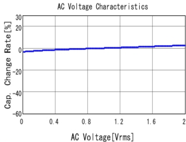
■ GRM319R71H334KA01 C-AC Voltage capchange, DCOV, 25.0d
