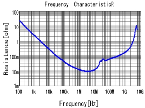
■ GRM319R71H334KA01 R DCOV, 25degC
