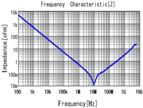
■ GRM319R71H334KA01 |Z| DCOV, 25degC
