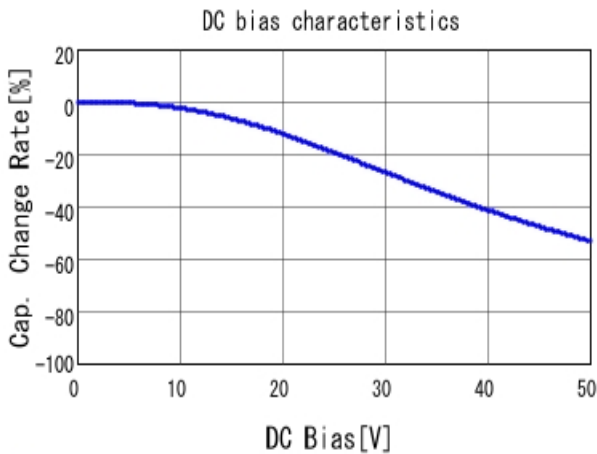
■ GRM319R71H334KA01 C-DC bias capchange, 25.0degC, AC1.
