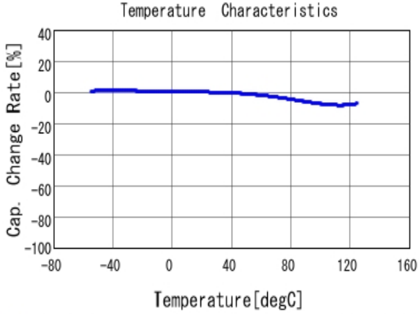
■ GRM319R71H334KA01 C-Temp. capchange, DC0.0V, AC1.0V r m
