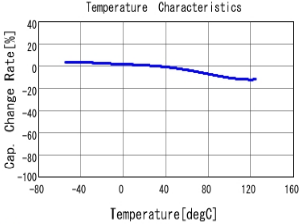
■ GRM319R71C105KAA3 C-Temp. capchange, DC0.0V, AC1.0V r m
