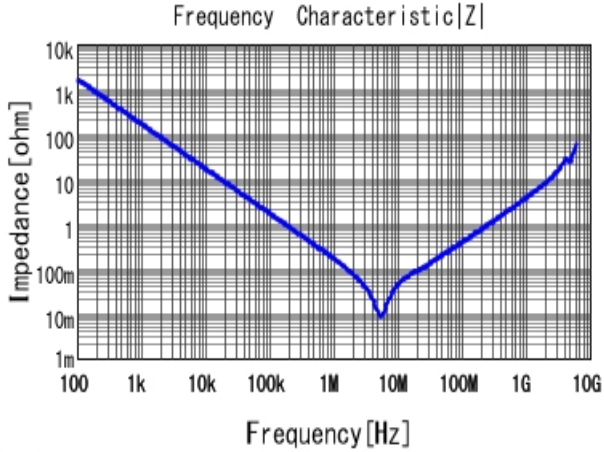
■ GRM319R71C105KAA3 |Z| DCOV, 25degC
