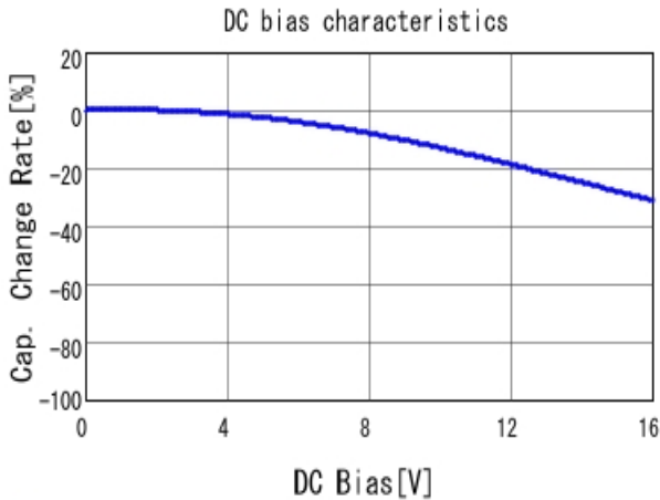
■ GRM319R71C105KAA3 C-DC bias capchange, 25.0degC, AC1.
