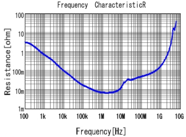
■ GRM319R71C105KAA3 R DCOV, 25degC
