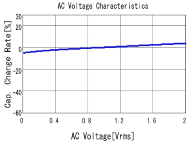
■ GRM319R71C105KAA3 C-AC Voltage capchange, DCOV, 25.0d
