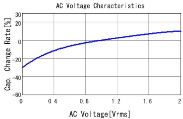
GRM319R61E475KA12 C-AC Voltage capchange, DCOV, 25
