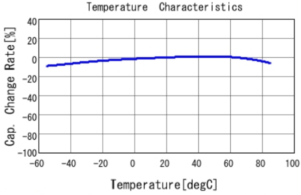
GRM319R61E475KA12 C-Temp. capchange, DC0.0V, AC1.C
