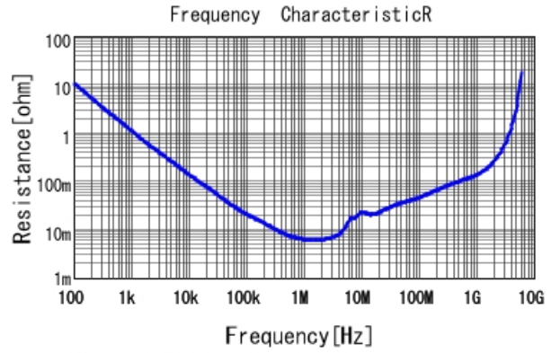
GRM319R61E475KA12 R DCOV, 25degC
