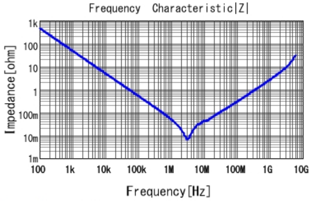
GRM319R61E475KA12 |Z| DCOV, 25degC
