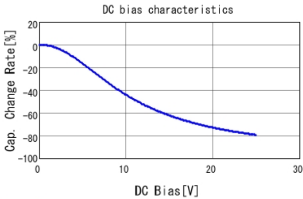
GRM319R61E475KA12 C-DC bias capchange, 25.0degC, A
