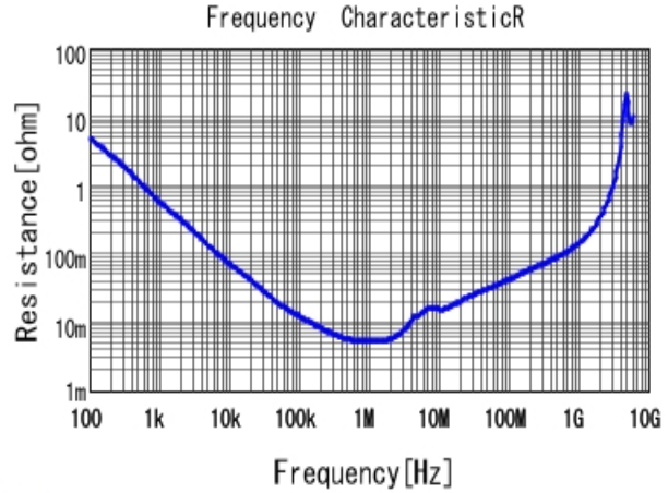
■ GRM319R61C106KE15 R DCOV, 25degC
