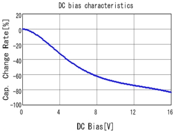
■ GRM319R61C106KE15 C-DC bias capchange, 25.0degC, AC0.
