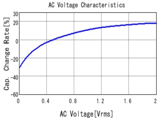
■ GRM319R61C106KE15 C-AC Voltage capchange, DCOV, 25.0d
