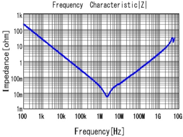
■ GRM319R61C106KE15 |Z| DCOV, 25degC
