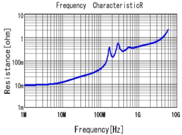
■ GRM3195C2A472JA01 R DCOV, 25degC
