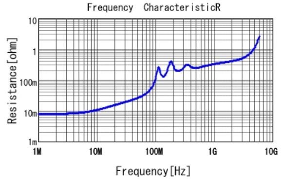
■ GRM3195C2A103JA01 R DCOV, 25degC
