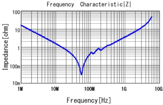
■ GRM3195C2A103JA01 |Z| DCOV, 25degC
