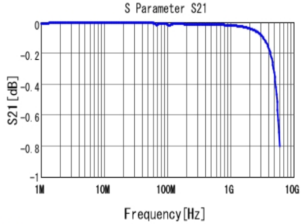
■ GRM3195C1H333JA01 S21 DCOV, 25degC
