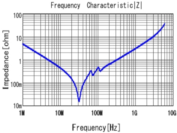
■ GRM3195C1H333JA01 |Z| DCOV, 25degC
