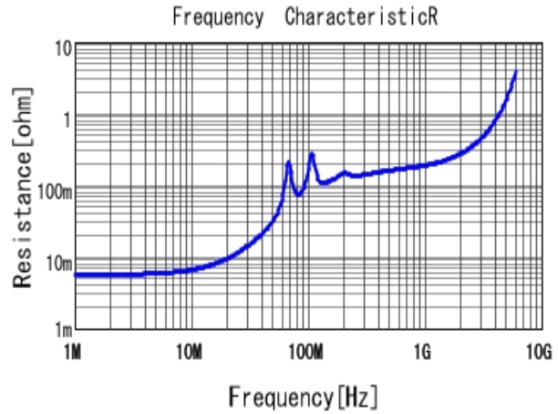
■ GRM3195C1H333JA01 R DCOV, 25degC
