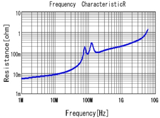
■ GRM3195C1H273JA01 R DCOV, 25degC
