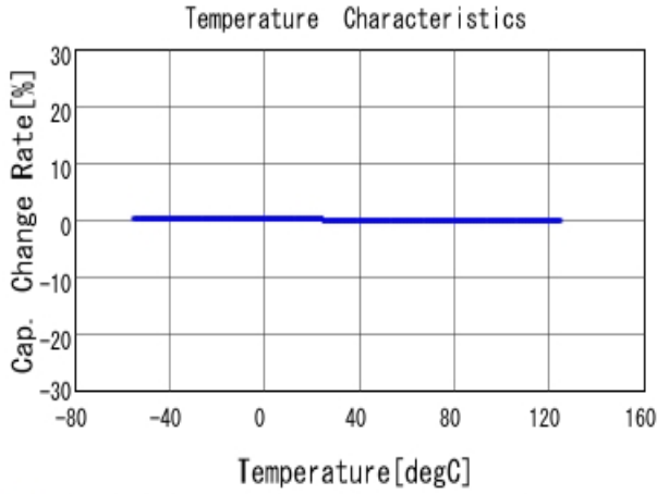
■ GRM3195C1H273JA01 C-Temp. capchange, DCOV, AC1Vrms
