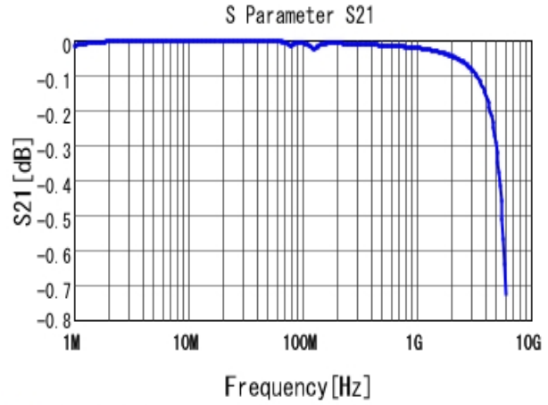
■ GRM3195C1H273JA01 S21 DCOV, 25degC
