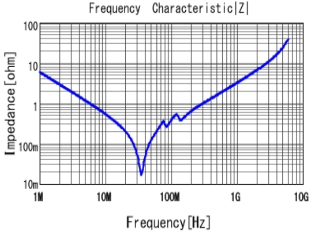
■ GRM3195C1H273JA01 |Z| DCOV, 25degC
