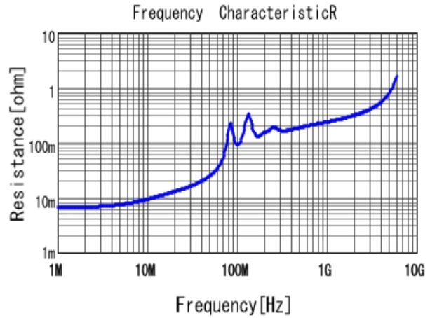
■ GRM3195C1H223JA01 R DCOV, 25degC
