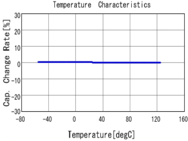
■ GRM3195C1H103JA01 C-Temp. capchange, DCOV, AC1Vrms
