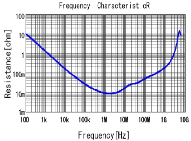
■ GRM316R61A475KE19 R DCOV, 25degC
