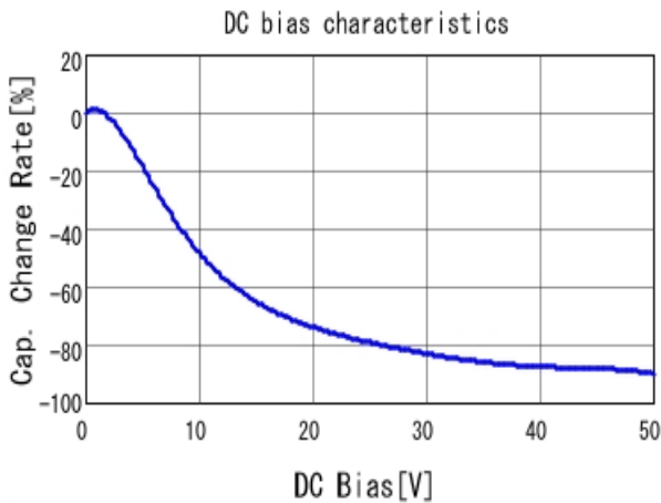
■ GRM21BZ71H475KE15 C-DC bias capchange, 25.0degC, AC1V
