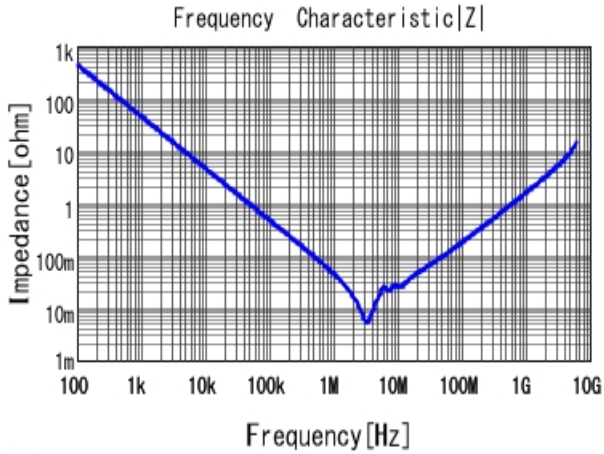
■ GRM21BZ71H475KE15 |Z| DCOV, 25degC
