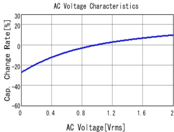
■ GRM21BZ71H475KE15 C-AC Voltage capchange, DCOV, 25.0d
