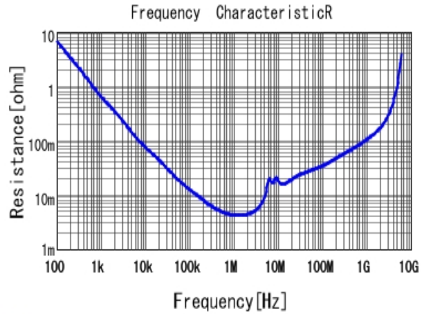
■ GRM21BZ71H475KE15 R DCOV, 25degC
