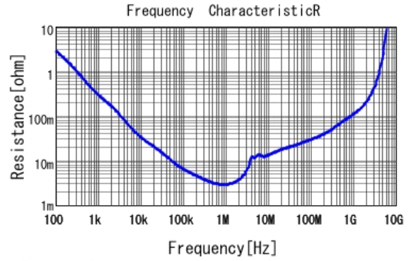
■ GRM21BZ71E106KE15 R DCOV, 25degC
