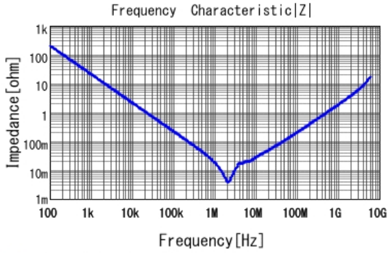
■ GRM21BZ71E106KE15 |Z| DCOV, 25degC
