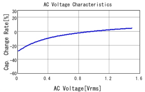
■ GRM21BZ71E106KE15 C-AC Voltage capchange, DCOV, 25.0d
