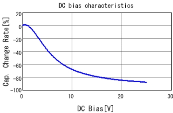
■ GRM21BZ71E106KE15 C-DC bias capchange, 25.0degC, AC1V
