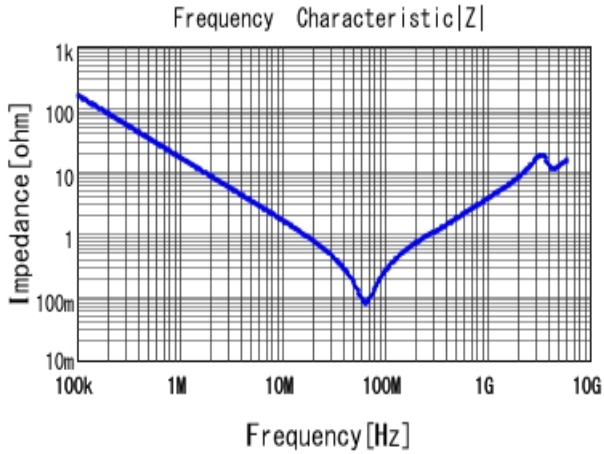
■ GRM21BR72E103KW03 |Z| DCOV, 25degC
