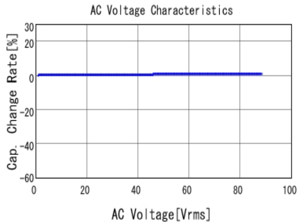
■ GRM21BR72E103KW03 C-AC Voltage capchange, DCOV, 25.0d
