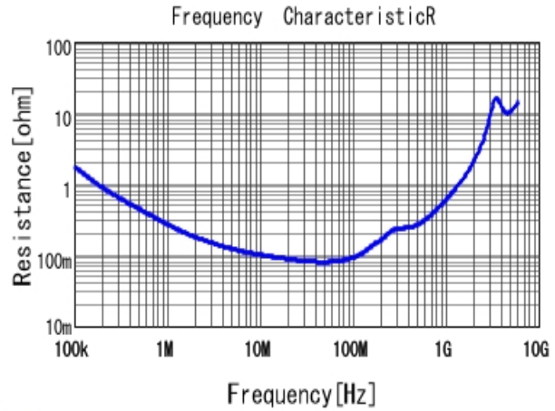
■ GRM21BR72E103KW03 R DCOV, 25degC
