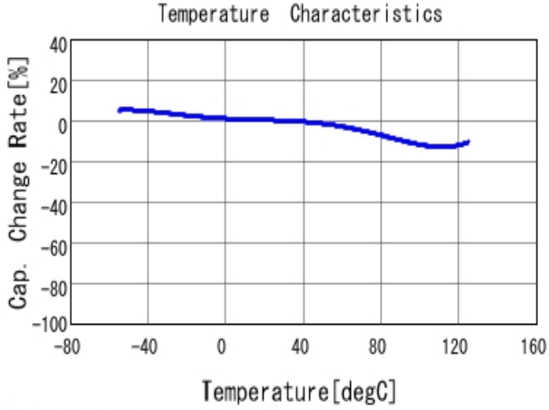
■ GRM21BR72E103KW03 C-Temp. capchange, DCOV, AC1Vrms
