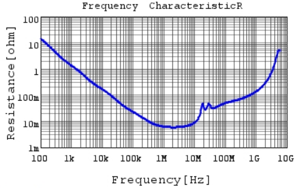
GRM21BR72A474KA73 R DCOV, 25degC
