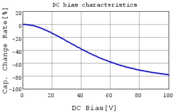
GRM21BR72A474KA73 C-DC bias capchange, 25.0c
