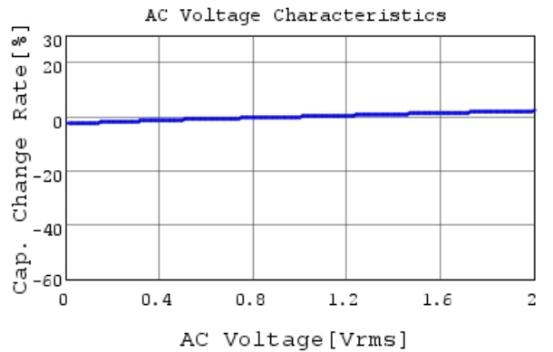
GRM21BR72A474KA73 C-AC Voltage capchange, Dc
