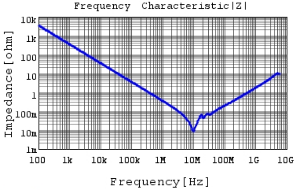
GRM21BR72A474KA73 |Z| DCOV, 25degC
