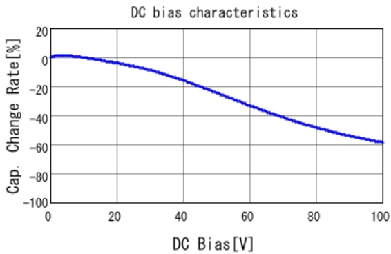
■ GRM21BR72A473KA01 C-DC bias capchange, 25.0degC, AC1.
