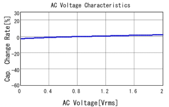
■ GRM21BR72A473KA01 C-AC Voltage capchange, DCOV, 25.0d
