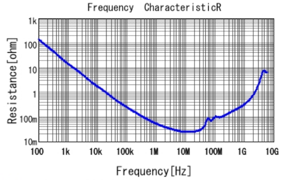
■ GRM21BR72A473KA01 R DCOV, 25degC
