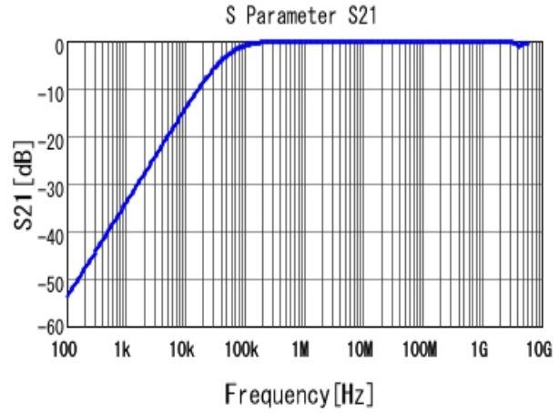
■ GRM21BR72A333KA01 S21 DC0V, 25degC
