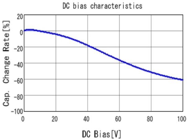
■ GRM21BR72A333KA01 C-DC bias capchange, 25.0degC, AC1.
