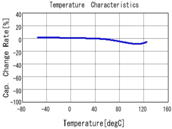
■ GRM21BR72A333KA01 C-Temp. capchange, DC0.0V, AC1.0V rm
