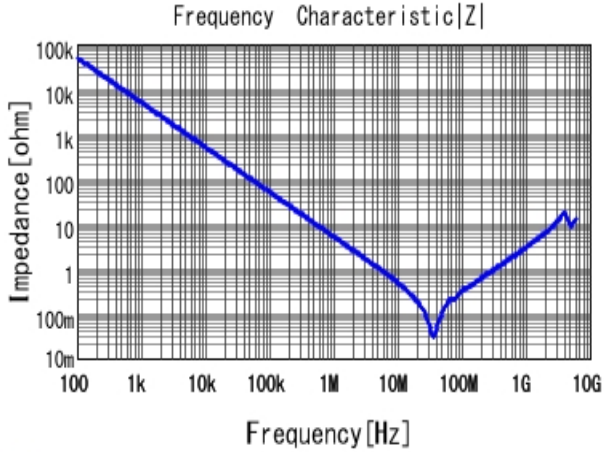
■ GRM21BR72A333KA01 |Z| DCOV, 25degC
