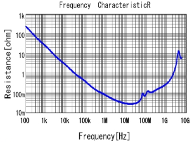
■ GRM21BR72A333KA01 R DCOV, 25degC
