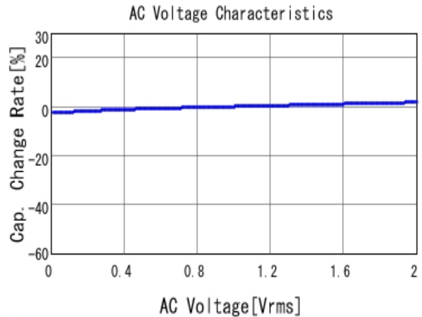
■ GRM21BR72A333KA01 C-AC Voltage capchange, DCOV, 25.0d
