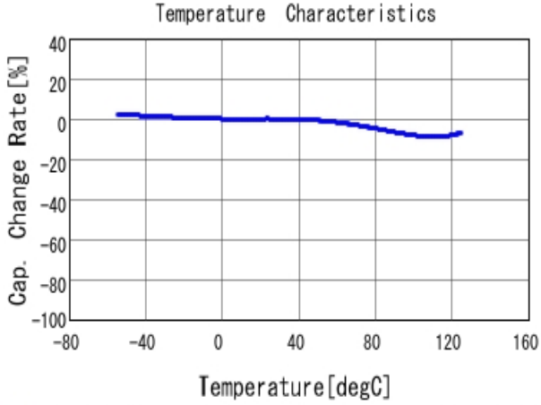
■ GRM21BR72A104KAC4 C-Temp. capchange, DC0.0V, AC1.0V rm
