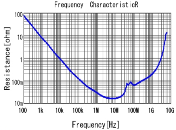
■ GRM21BR72A104KAC4 R DCOV, 25degC
