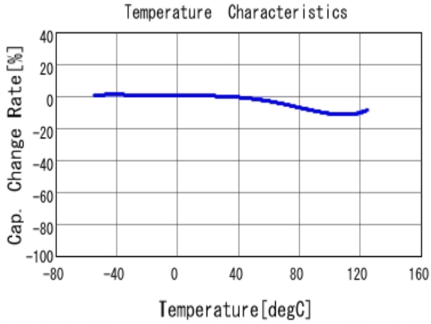
■ GRM21BR71H473KA01 C-Temp. capchange, DCO. 0V, AC1.0Vrm
