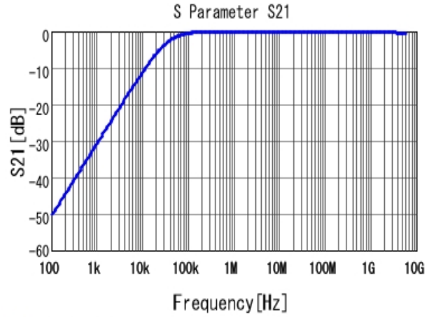
■ GRM21BR71H473KA01 S21 DCOV, 25degC
