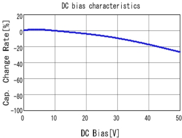
■ GRM21BR71H473KA01 C-DC bias capchange, 25.0degC, AC1.
