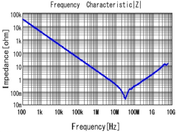
■ GRM21BR71H473KA01 |Z| DCOV, 25degC
