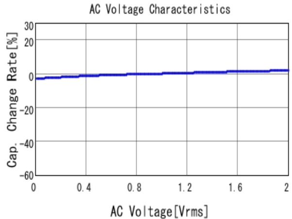
■ GRM21BR71H473KA01 C-AC Voltage capchange, DCOV, 25.0d
