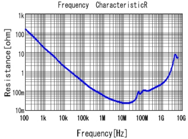
■ GRM21BR71H473KA01 R DCOV, 25degC
