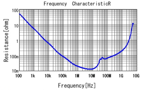
■ GRM21BR71H154KA01 R DCOV, 25degC
