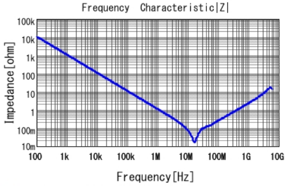
■ GRM21BR71H154KA01 |Z| DCOV, 25degC
