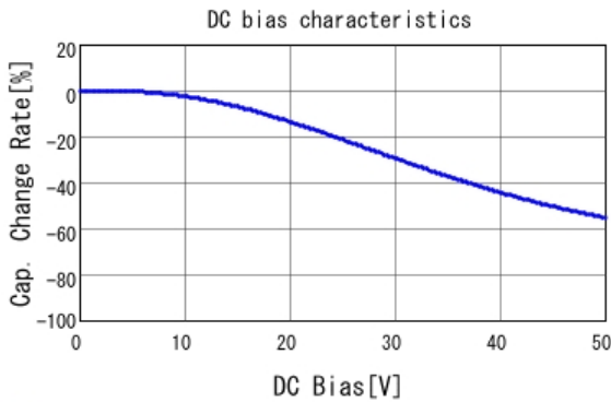
■ GRM21BR71H154KA01 C-DC bias capchange, 25.0degC, AC1.
