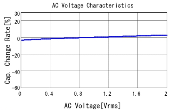
■ GRM21BR71H154KA01 C-AC Voltage capchange, DCOV, 25.0d
