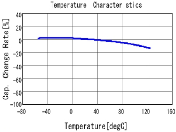
■ GRM21BR71H105KA12 C-Temp. capchange, DC0.0V, AC1.0V r m
