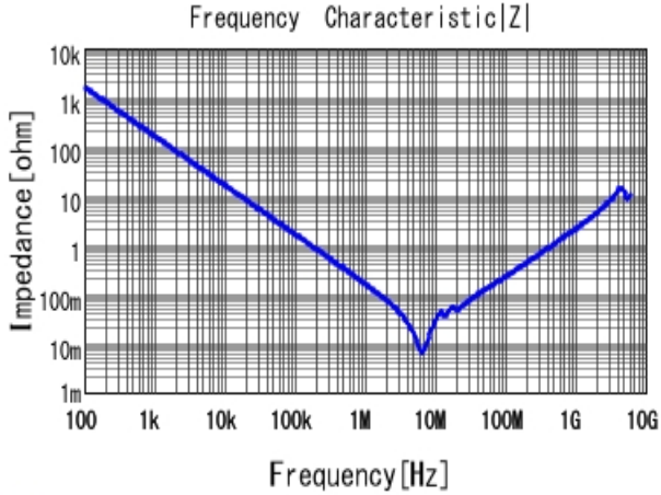
■ GRM21BR71H105KA12 |Z| DCOV, 25degC
