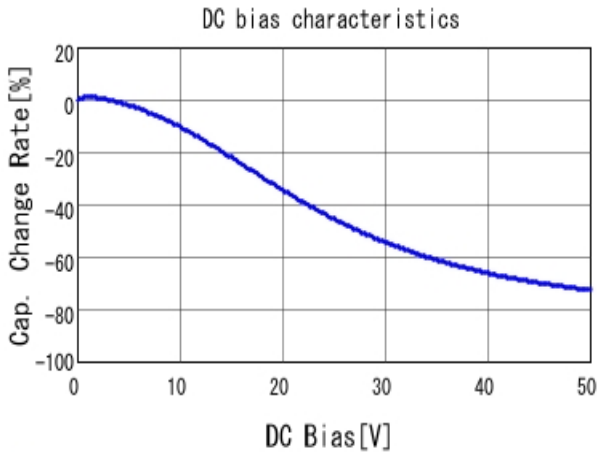
■ GRM21BR71H105KA12 C-DC bias capchange, 25.0degC, AC1.
