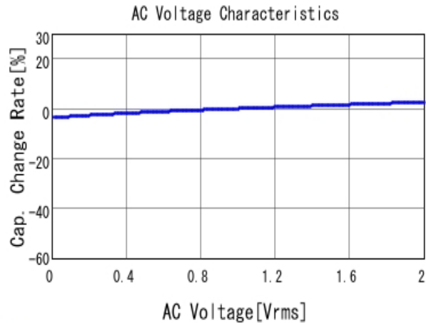
■ GRM21BR71H105KA12 C-AC Voltage capchange, DCOV, 25.0d
