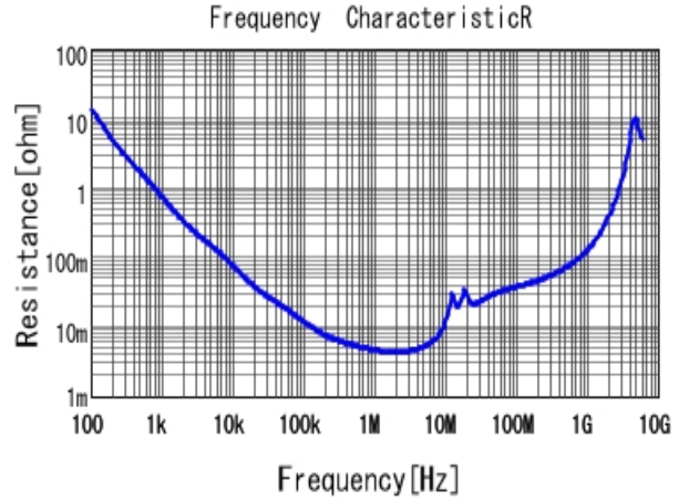
■ GRM21BR71H105KA12 R DCOV, 25degC
