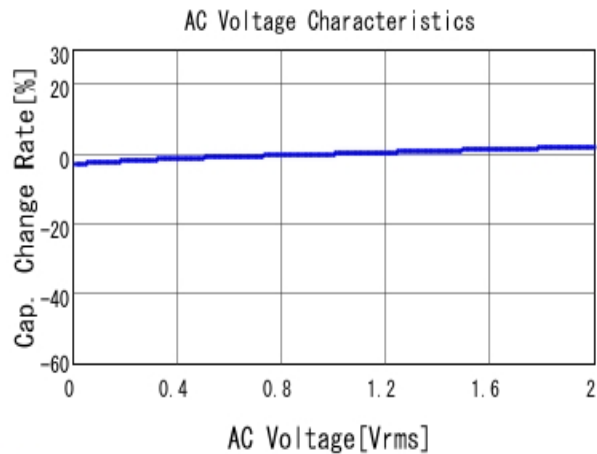
■ GRM21BR71H104KA01 C-AC Voltage capchange, DCOV, 25.0d
