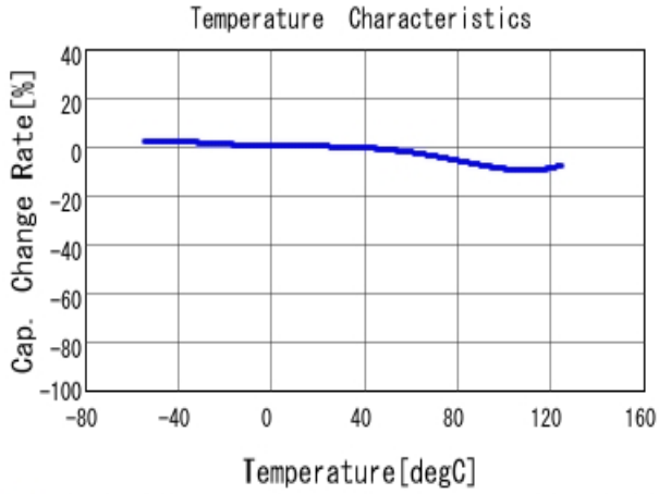
■ GRM21BR71H104KA01 C-Temp. capchange, DC0.0V, AC1.0V rm
