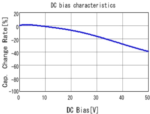
■ GRM21BR71H104KA01 C-DC bias capchange, 25.0degC, AC1.
