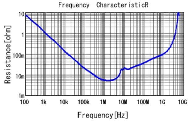
GRM21BR71E475KA73 R DCOV, 25degC
