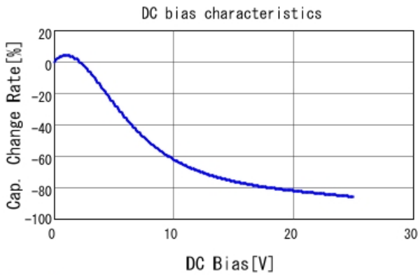
GRM21BR71E475KA73 C-DC bias capchange, 25.0degC, A
