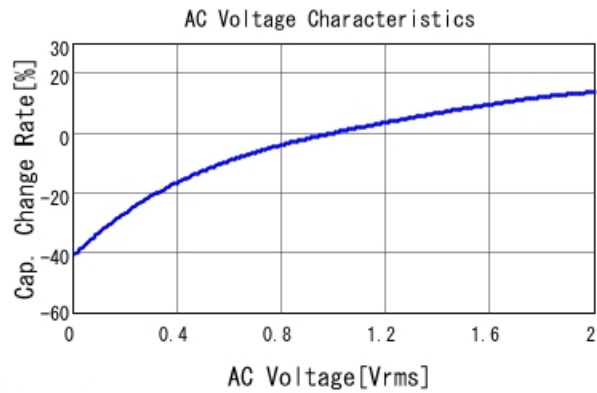
GRM21BR71E475KA73 C-AC Voltage capchange, DCOV, 25
