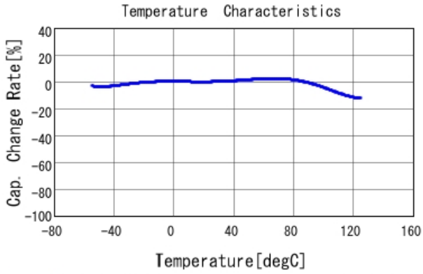
GRM21BR71E475KA73 C-Temp. capchange, DC0.0V, AC1.C
