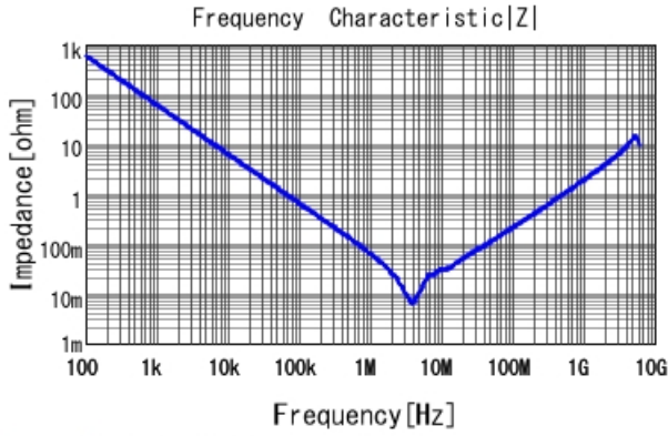
GRM21BR71E475KA73 |Z| DCOV, 25degC
