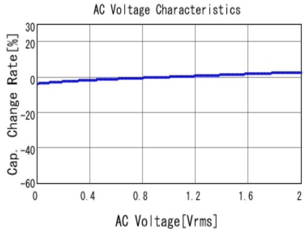
■ GRM21BR71E334KA01 C-AC Voltage capchange, DCOV, 25.0d
