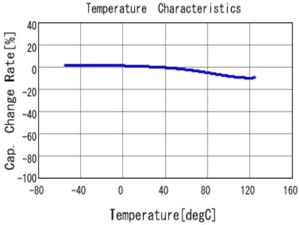
■ GRM21BR71E334KA01 C-Temp. capchange, DC0.0V, AC1.0V r m
