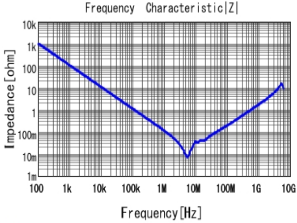
■ GRM21BR71E225KE11 |Z| DCOV, 25degC
