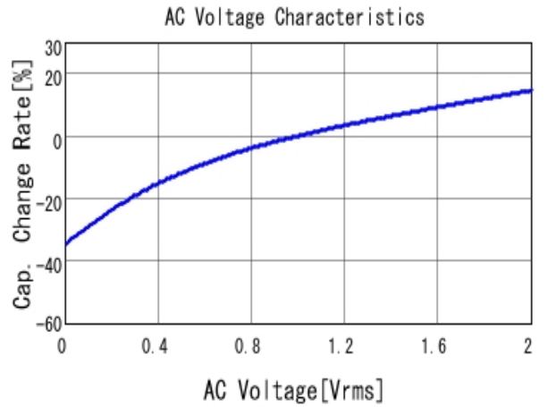
■ GRM21BR71E225KE11 C-AC Voltage capchange, DCOV, 25.0d
