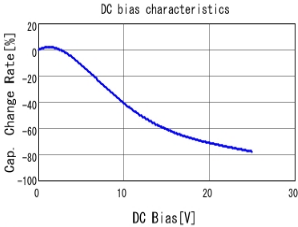
■ GRM21BR71E225KE11 C-DC bias capchange, 25.0degC, AC1V
