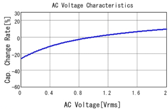
■ GRM21BR71E225KA73 C-AC Voltage capchange, DCOV, 25.0d
