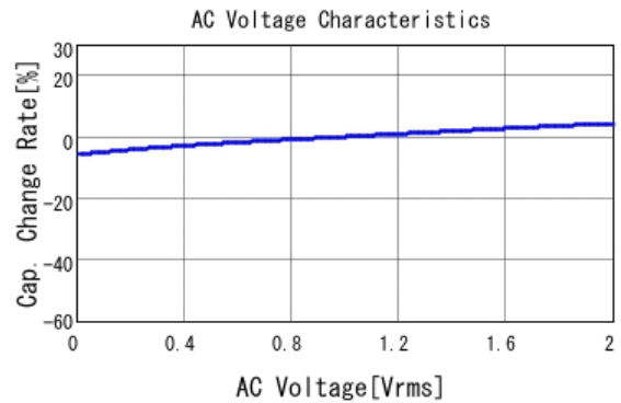
■ GRM21BR71E105KA99 C-AC Voltage capchange, DCOV, 25.0d
