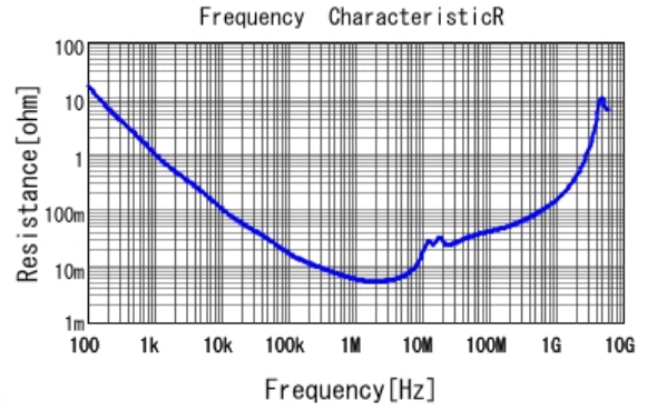
■ GRM21BR71E105KA99 R DCOV, 25degC
