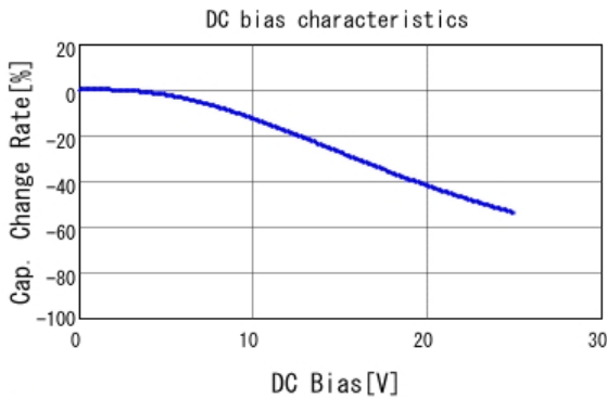
■ GRM21BR71E105KA99 C-DC bias capchange, 25.0degC, AC1.
