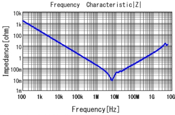
■ GRM21BR71E105KA99 |Z| DCOV, 25degC
