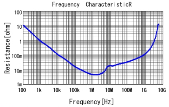
■ GRM21BR71C475KE51 R DCOV, 25degC
