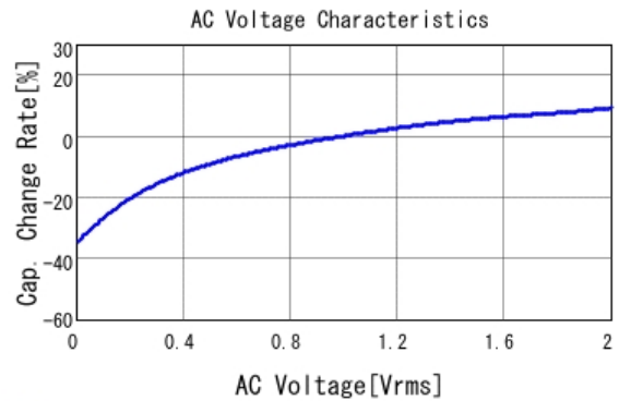
■ GRM21BR71C475KE51 C-AC Voltage capchange, DCOV, 25.0d
