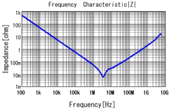
■ GRM21BR71C475KE51 |Z| DCOV, 25degC
