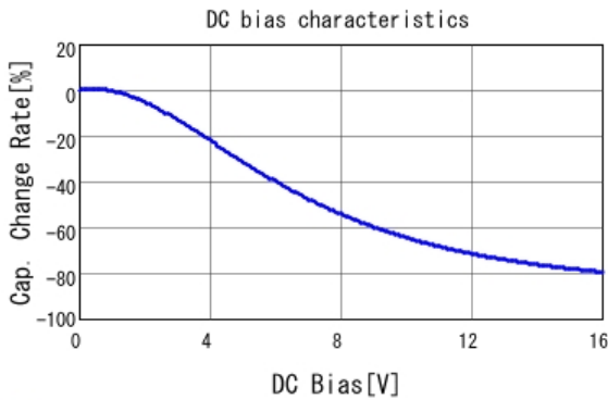
■ GRM21BR71C475KE51 C-DC bias capchange, 25.0degC, AC1V
