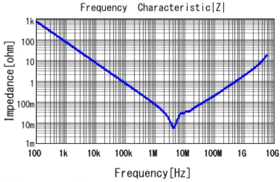
■ GRM21BR71C225KA12 |Z| DCOV, 25degC
