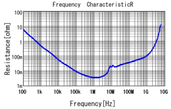
■ GRM21BR71C225KA12 R DCOV, 25degC
