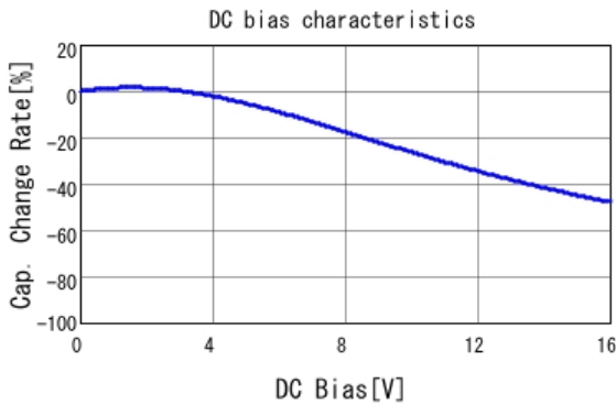
■ GRM21BR71C225KA12 C-DC bias capchange, 25.0degC, AC1.
