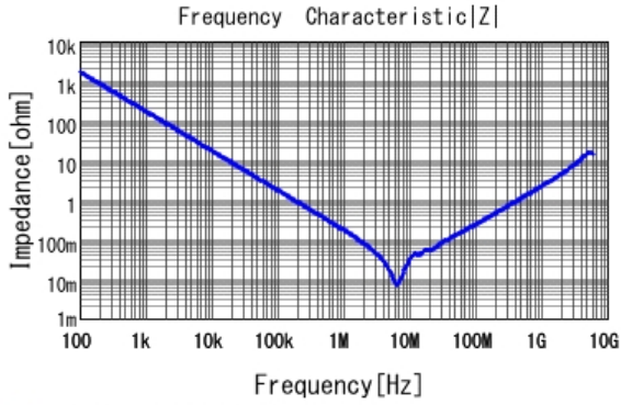
■ GRM21BR71C105KA01 |Z| DCOV, 25degC
