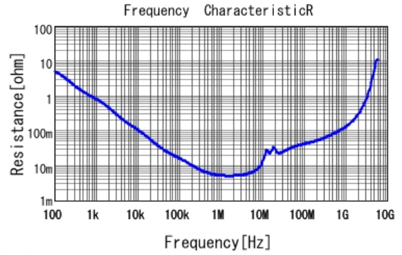
■ GRM21BR71C105KA01 R DCOV, 25degC
