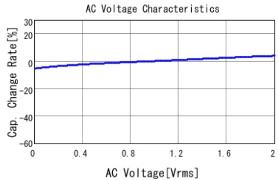
■ GRM21BR71C105KA01 C-AC Voltage capchange, DCOV, 25.0d
