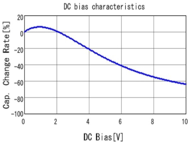
■ GRM21BR71A475KA73 C-DC bias capchange, 25.0degC, AC1.
