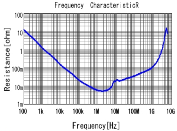
■ GRM21BR71A475KA73 R DCOV, 25degC
