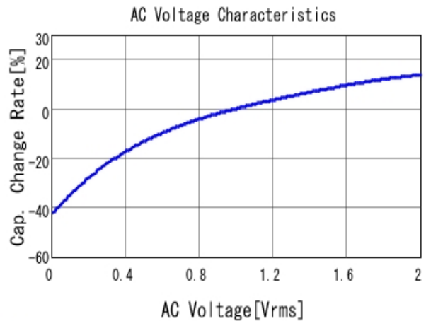
■ GRM21BR71A475KA73 C-AC Voltage capchange, DCOV, 25.0d
