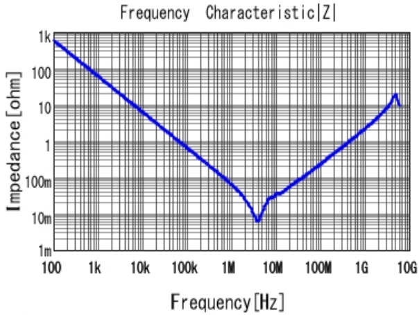
■ GRM21BR71A475KA73 |Z| DCOV, 25degC
