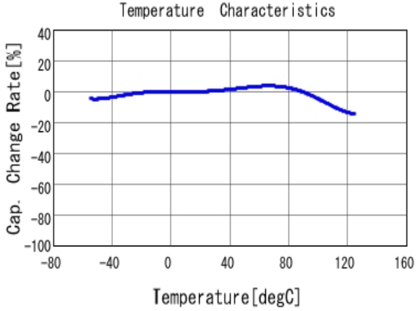
■ GRM21BR71A475KA73 C-Temp. capchange, DCO. 0V, AC1.0V rm
